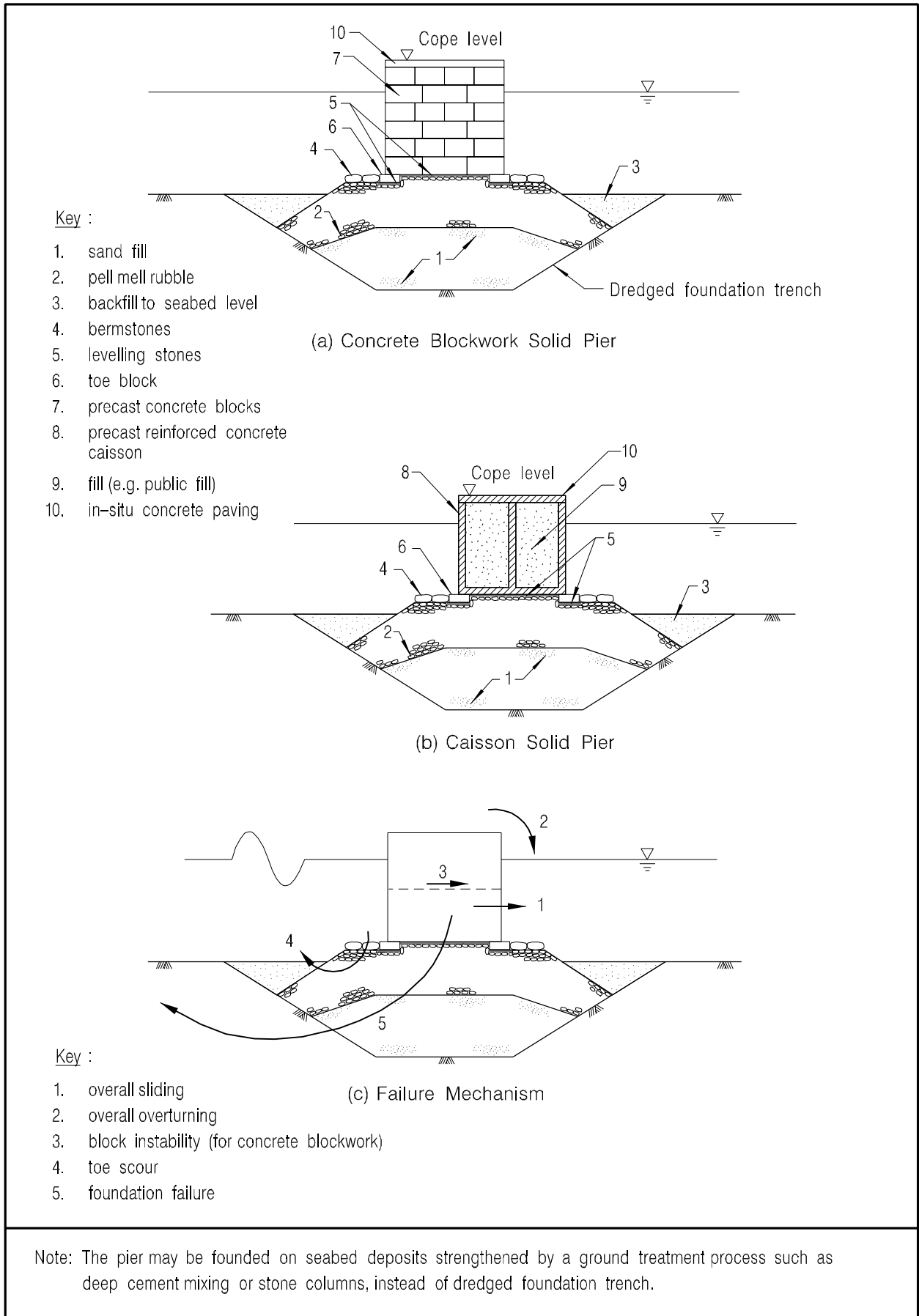
Figure 14 – Key Elements and Failure Mechanism of Solid Pier
