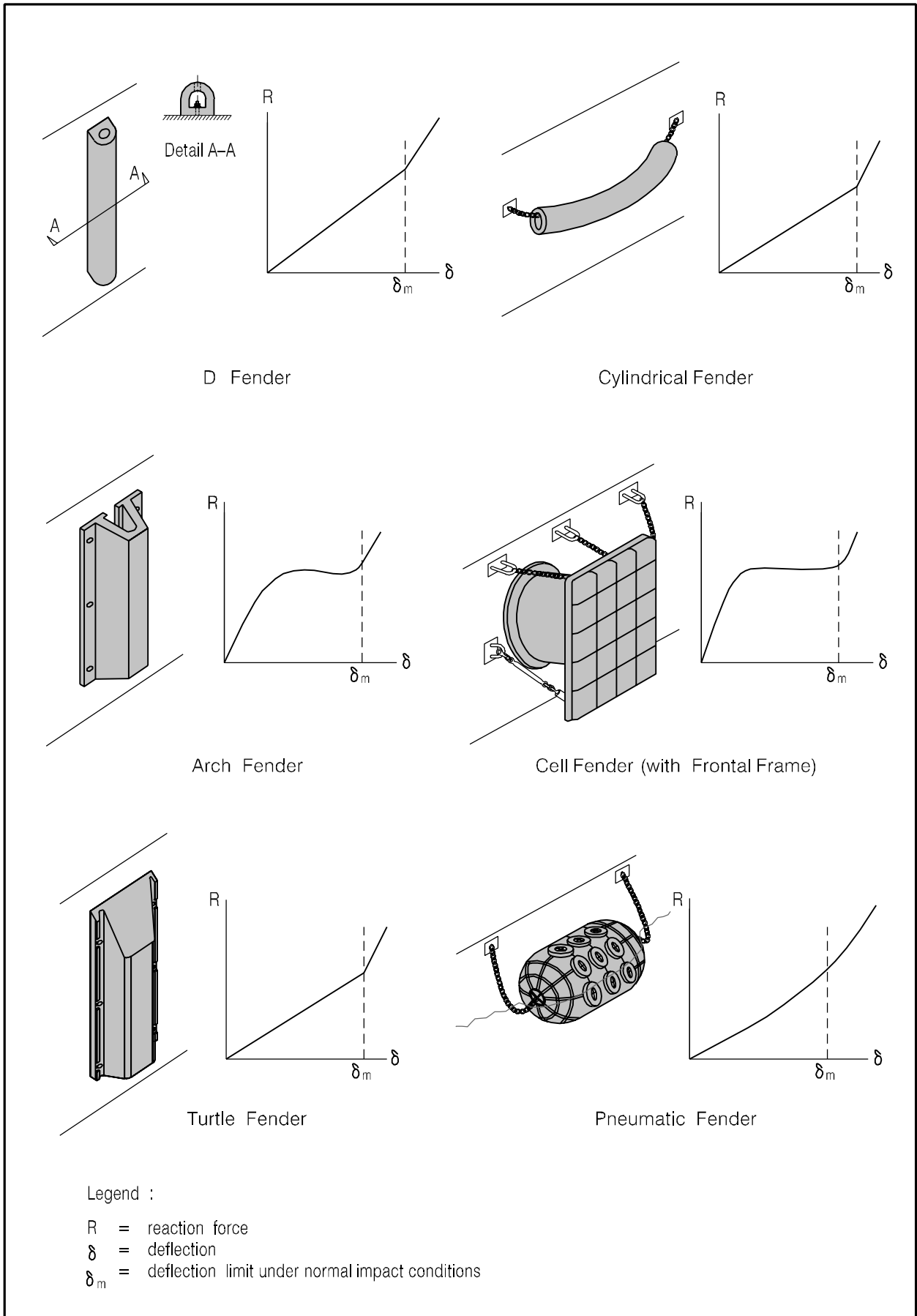
Figure 3 – Rubber Fenders
